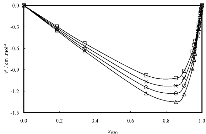
Figure 8. Excess molar volumes ( v^E ) for the (polyethylene glycol-400 + water) system at various temperatures determined in this work. Symbols: \square , 358.15 K; \times , 338.15 K; \circ , 318.15 K; \Delta , 298.15 K. Solid curves correlated values with eq 4 and parameters provided in Table 10.
